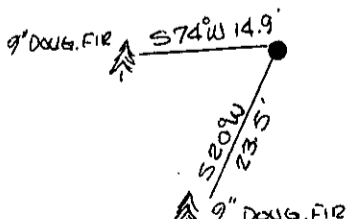
SKETCH OF CORNER
