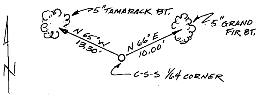
Decl. 18° SKETCH OF CORNER
