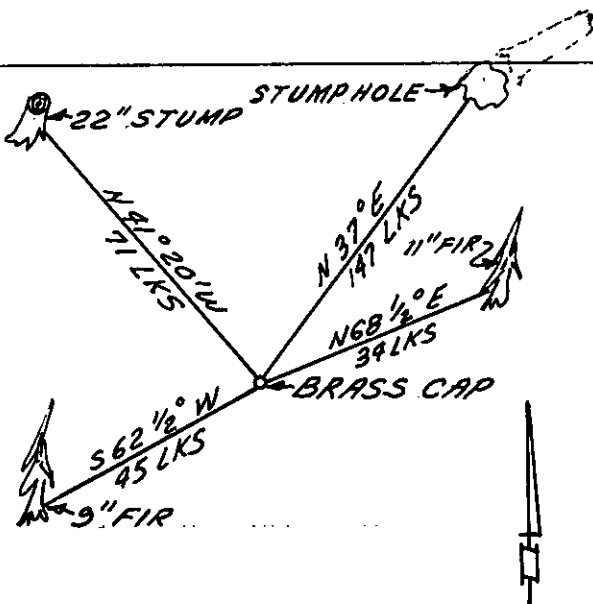
DIAGRAM OF CORNER
