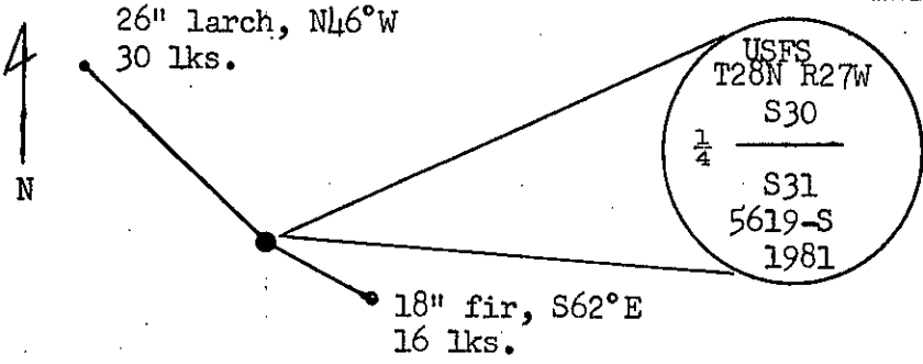
SKETCH OF CORNER No Scale
